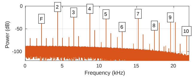
(c) 3rd order ADAA - linear interpolation - 8192-points LUT (SNR: 8.95 dB)
