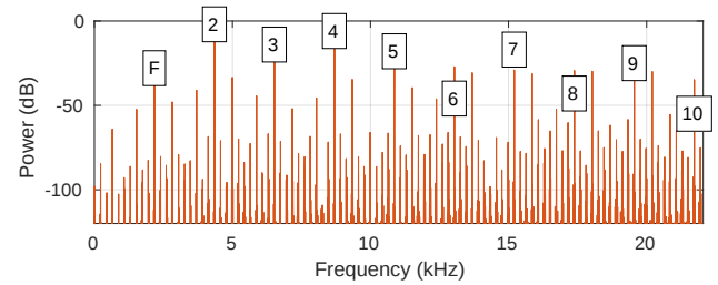
(b) 1st order ADAA - 8192-points LUT (SNR: 6.94 dB)
